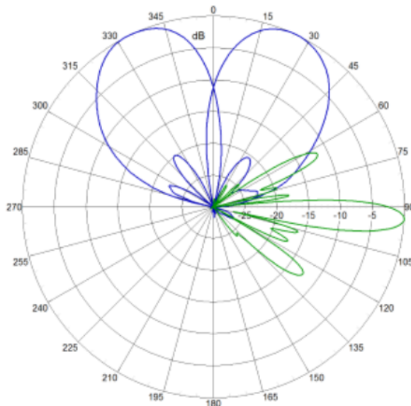
1940 MHz Azimuth Elevation 4°
