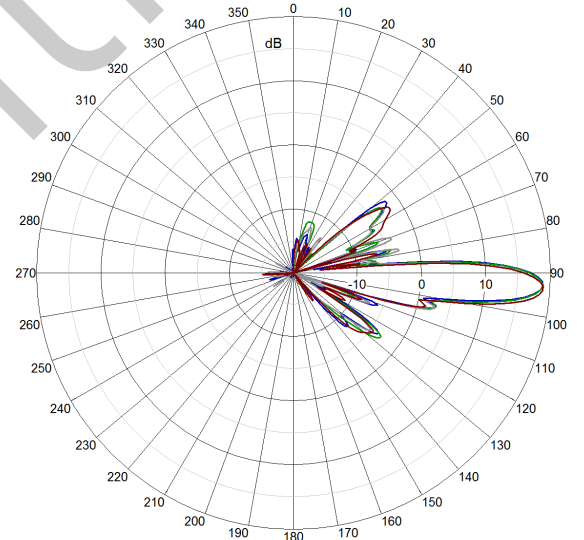
1940 MHz Elevation 4°
