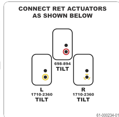
RET Connection Diagram
