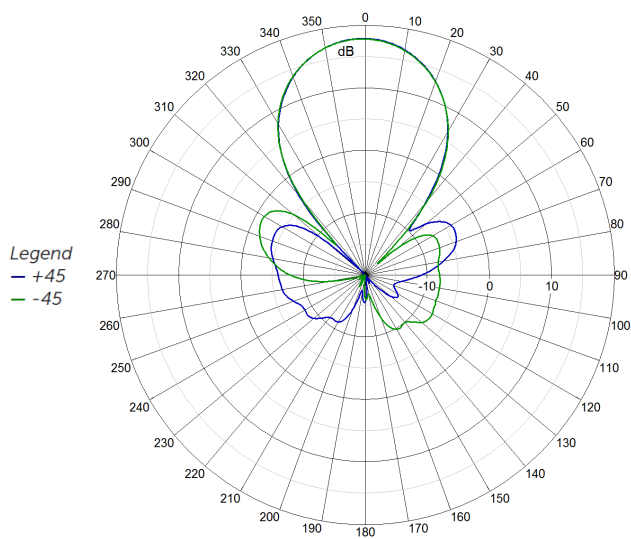
875 MHz Azimuth
