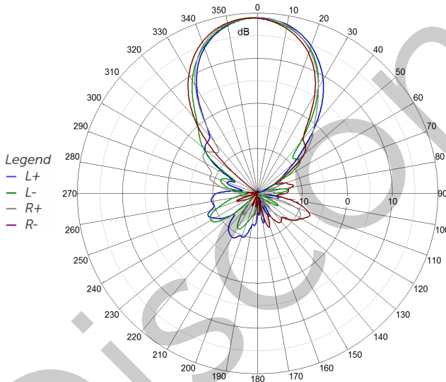
1940 MHz Azimuth
