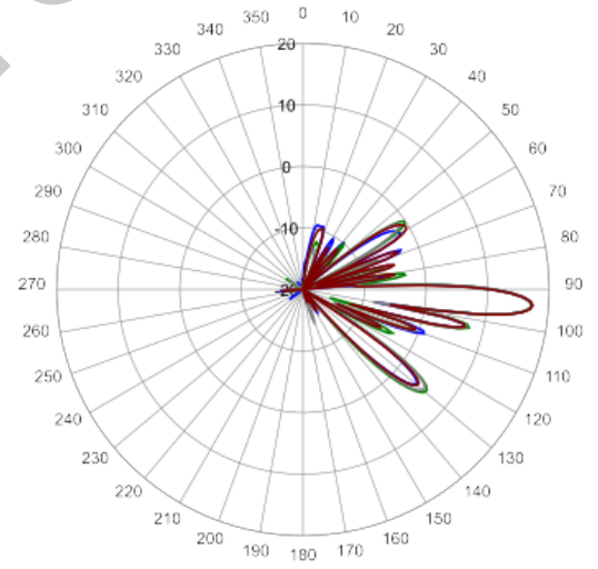
1930 MHz Elevation 4°
