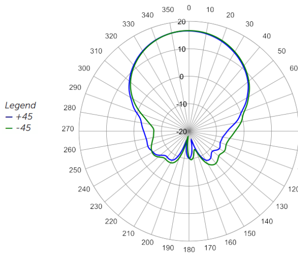
894 MHz Azimuth
